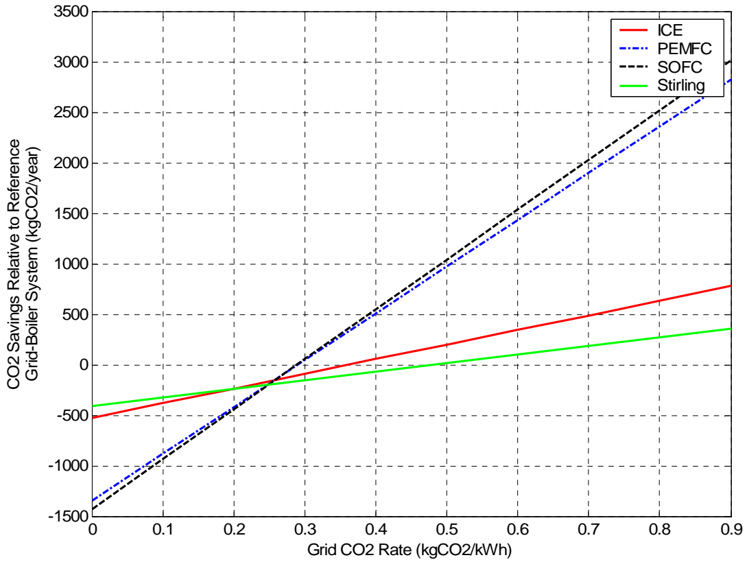
Figure 1: Sensitivity of Annual CO2 Emissions Reduction (kg CO2/year) to Emissions Credit Rate Granted for Onsite Generation (kg CO2/kWh) for 1kWe Micro-CHP Systems and Existing Terraced House Demand Scenario
