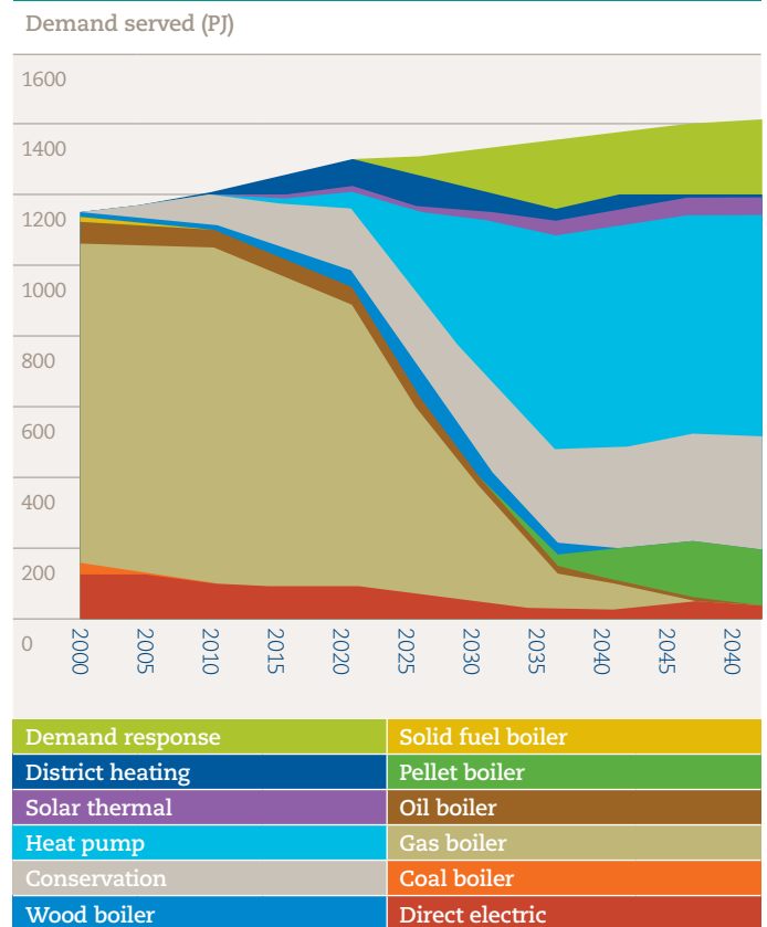
Figure 1: Demand Served by Residential Heating End-Use Technologies
