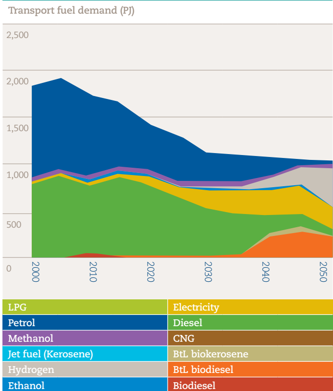
Figure 2: Energy Consumption in the Transport Sector in DECC-1A-IAB-2A
