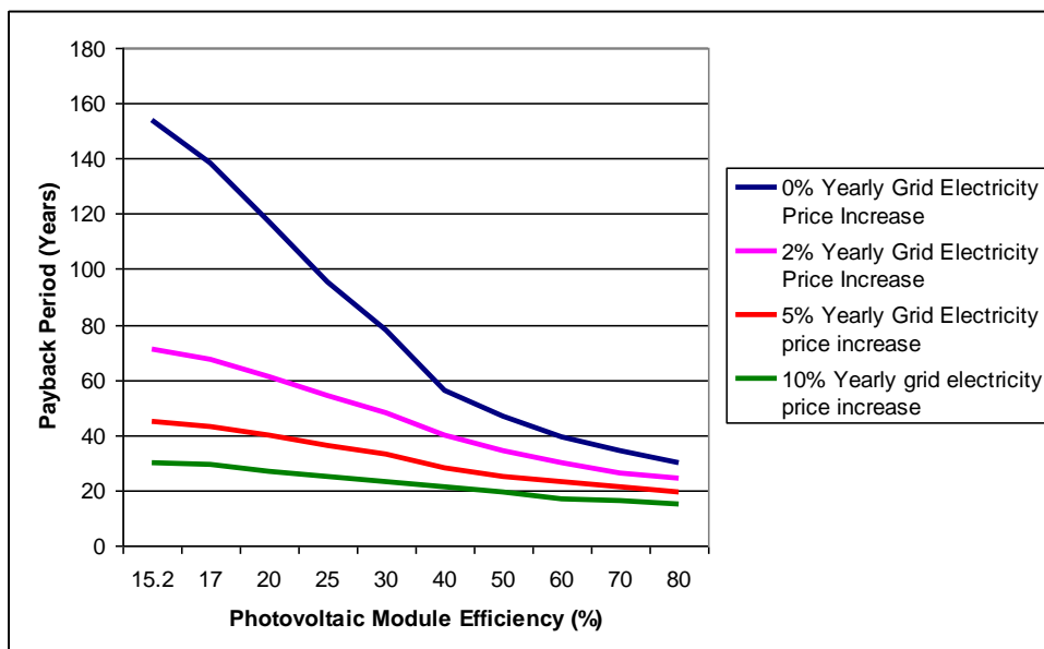
Figure 4: Payback period of a 20 kWp PV array for varying efficiencies and grid electricity price increases
