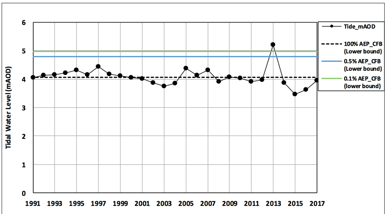
Figure 14. Extreme yearly tidal value (yearly maximum) at Immingham on the Humber (BODC tide gauge) and nearest CFB data (at chainage 3886 km) from different AEP events at lower bound of confidence interval. (Source: EA)
