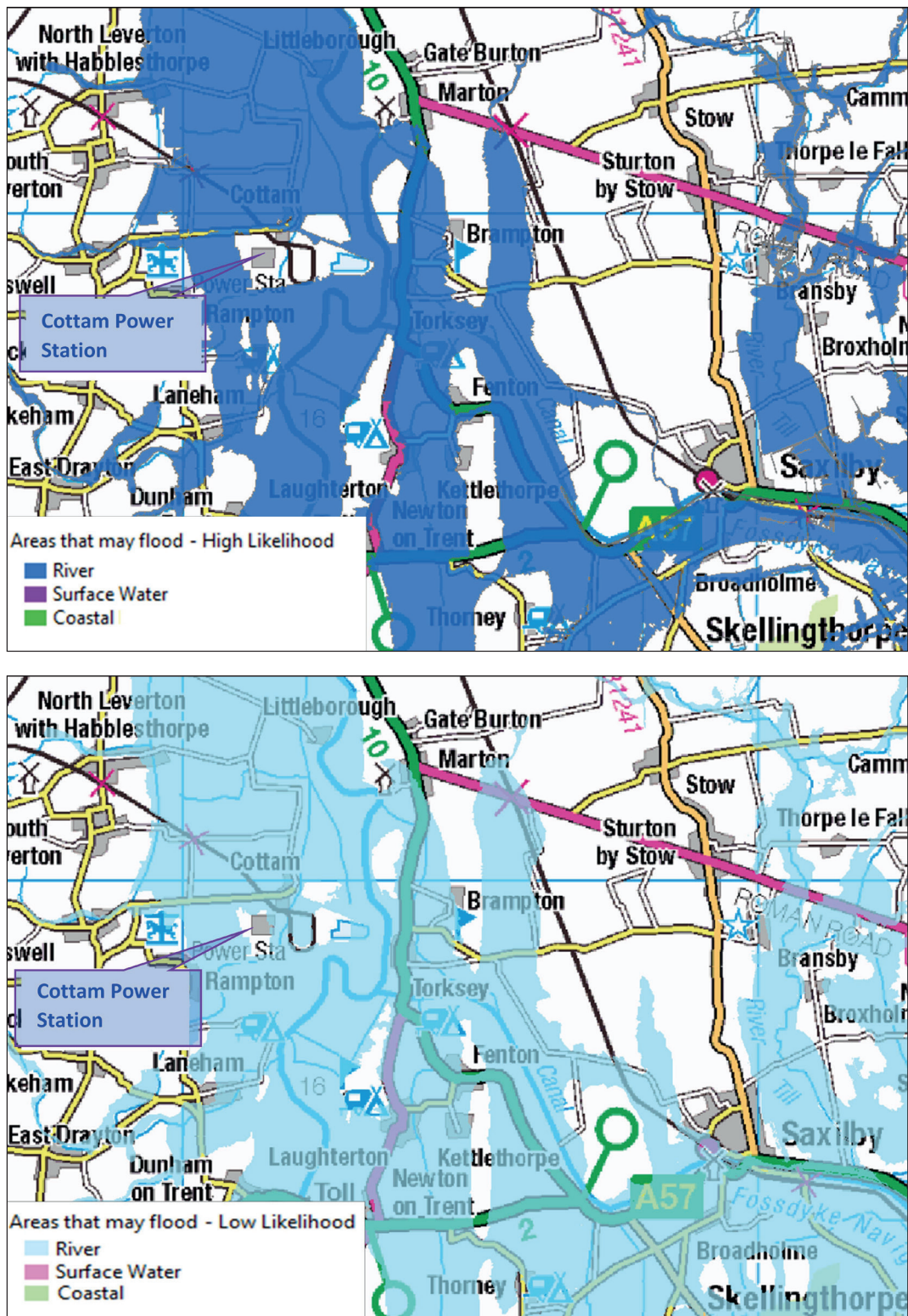
Figure 8. Zone 3 (high likelihood, upper plate) and Zone 2 (low likelihood, bottom plate) river flood outlines at Cottam. (Source: EA (contains Ordnance Survey data Crown copyright database right © 2018))
