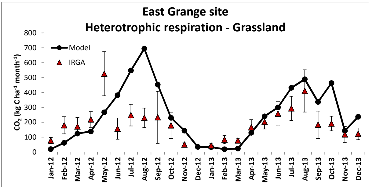
Figure 3.17: Soil heterotrophic respiration over the measured period; data from East Grange site. Heterotrophic respiration estimated from one dataset: IRGA = static chamber. Error bars represent 95% confidence interval of measured values.
